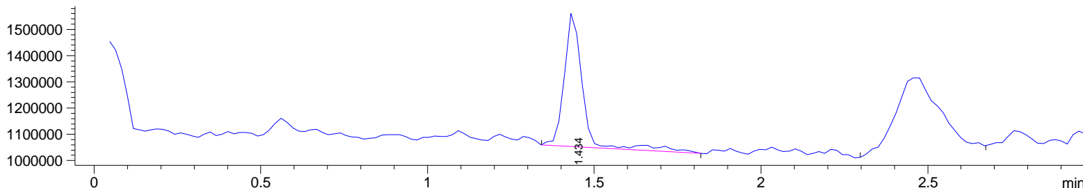
Integration Results for DAD1 A, Sig=214,4 Ref=360,100
